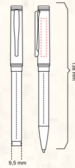
1520-RT ROLLER & TÜKENMEZ KALEM ROLLER & BALLPOINT PEN BASKI ALANI/PRINTING AREA Gövde/Body : 5 mm x 36 mm
