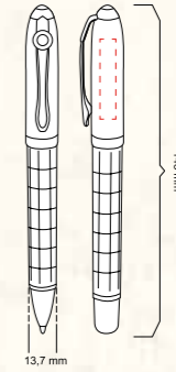
615-RT ROLLER & TÜKENMEZ KALEM ROLLER & BALLPOINT PEN BASKI ALANI/PRINTING AREA Gövde/Body : 5 mm x 28 mm
