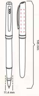
625-RT ROLLER & TÜKENMEZ KALEM ROLLER & BALLPOINT PEN BASKI ALANI/PRINTING AREA Gövde/Body : 5 mm x 32 mm
