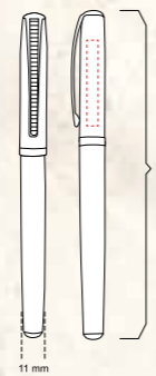
321-RT ROLLER & TÜKENMEZ KALEM ROLLER & BALLPOINT PEN BASKI ALANI/PRINTING AREA Gövde/Body : 5 mm x 34 mm
